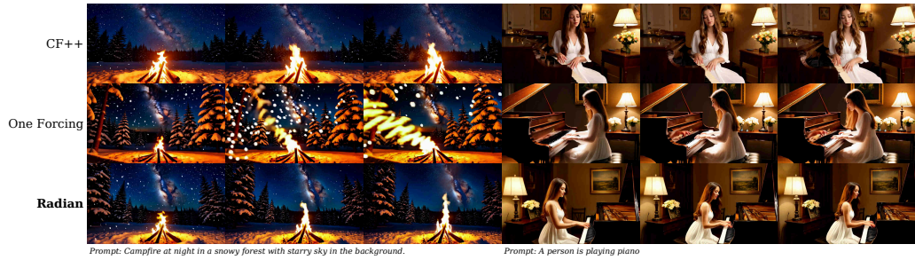
Figure 7: Additional one-step frame-wise comparisons. A snowy campfire and piano performance, with Causal Forcing++, One Forcing, and Radian arranged from top to bottom. The sampled frames show changes in scene appearance and subject framing.
