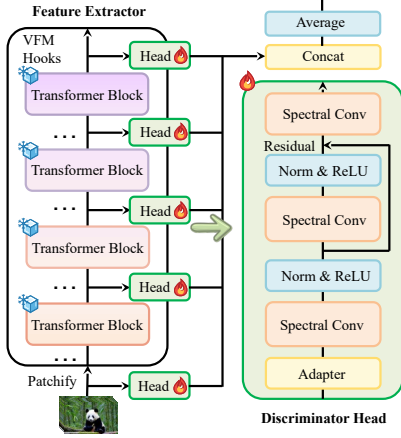
Figure 3: Architecture of Lightweight Discriminator Head.
