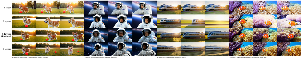
Figure 11: Feature-layer comparisons. Rows use one, two, four, and eight DINOv2-S feature layers, respectively. The cases show a corgi in a park, an astronaut, a train on tracks, and clownfish among coral; Radian uses the four-layer configuration.
