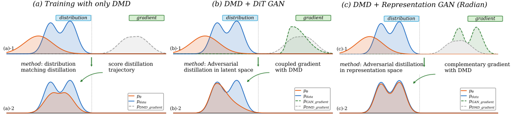
Figure 1: Complementary Representation-Space Supervision. Radian complements DMD with perceptual gradients, guiding the student toward a better-matched data distribution.
