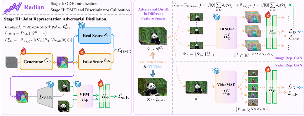
Figure 2: Overview of the Three-stage Training Pipeline.
